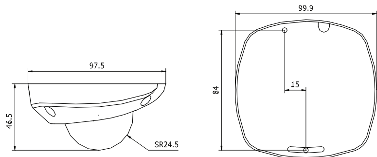
Indoor/Outdoor Wall Mount WMS + PC120
