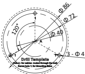
Figure 2. 9 Drill Template
