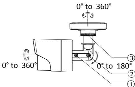
Figure 2. 3 3-Axis Adjustment
