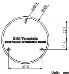
Figure 2. 5 Drill Template
